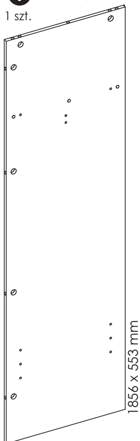
1 Bok lewy
